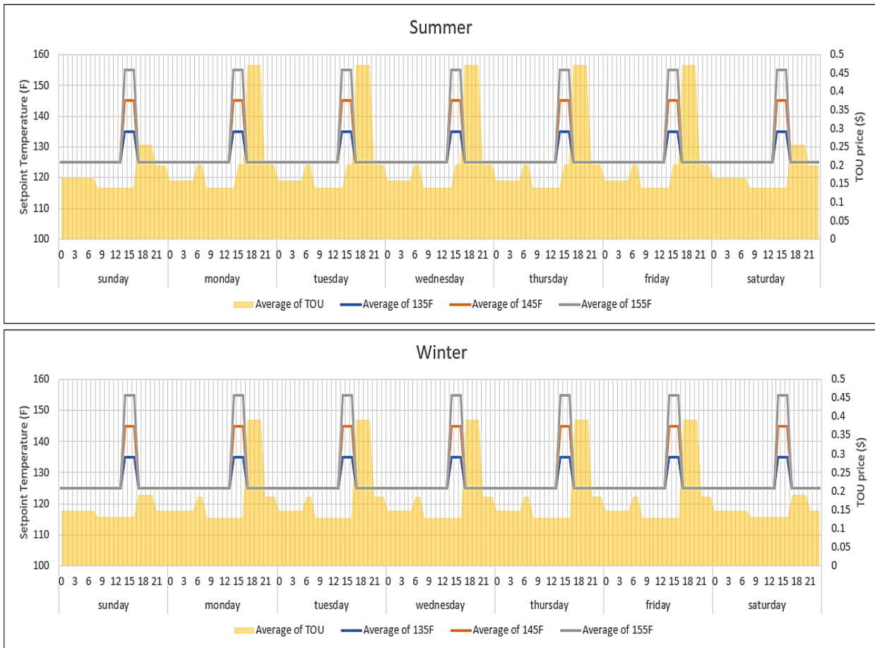
Figure 3. Load-up/shed strategy
