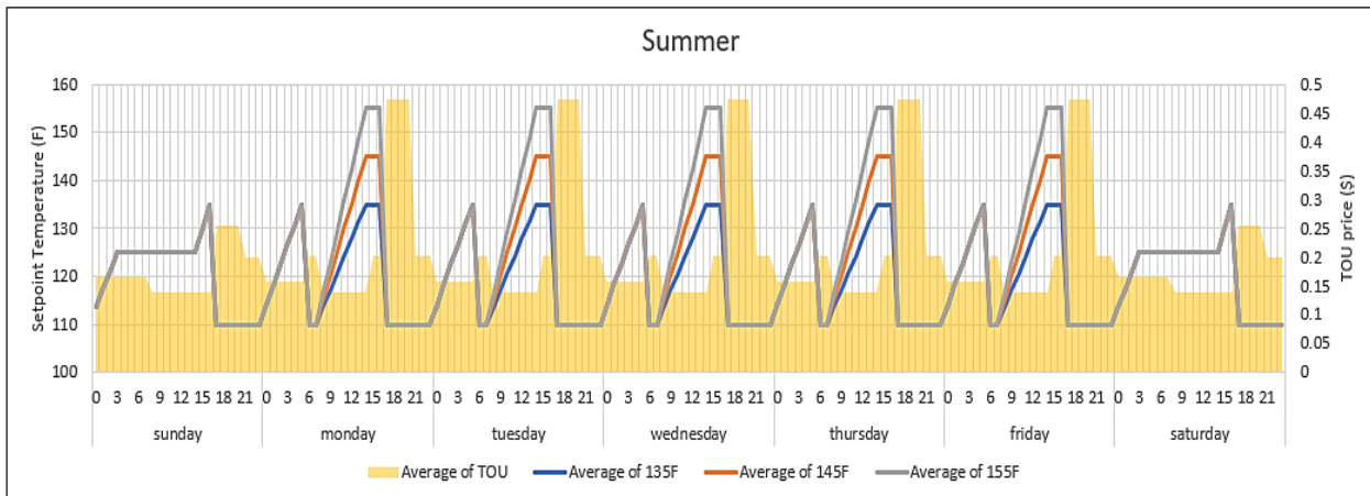
Figure 4. Load-up/Shed strategy.
